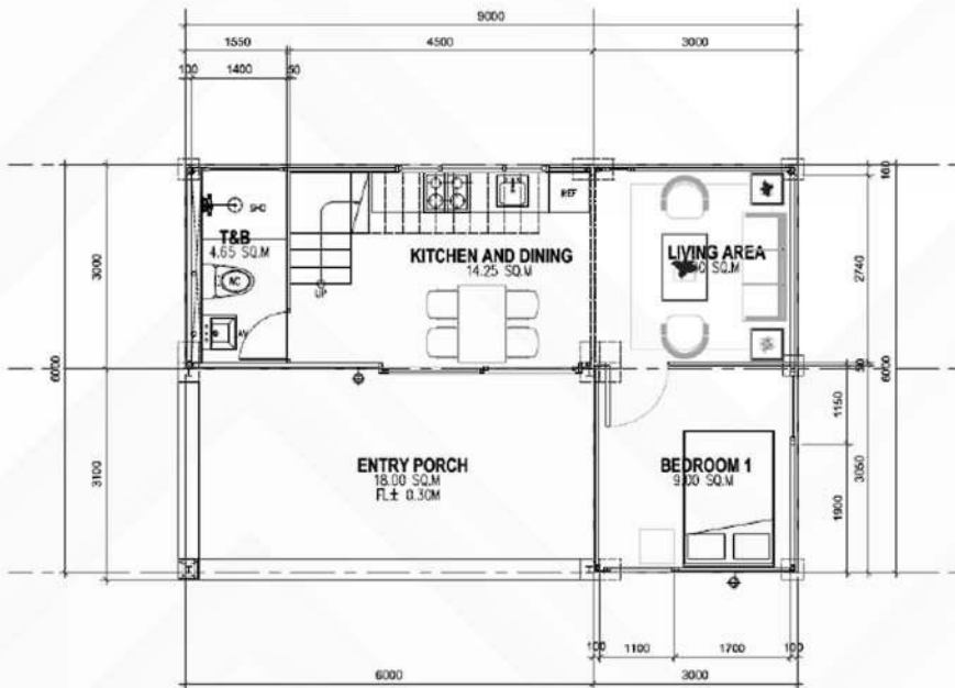
1 A1 GROUND FLOOR PLAN SCALE 1:50
