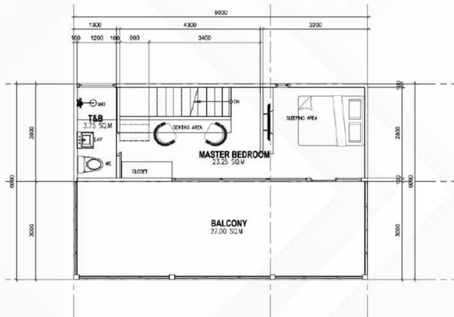
1 A2 SECOND FLOOR PLAN SCALE 1:50
